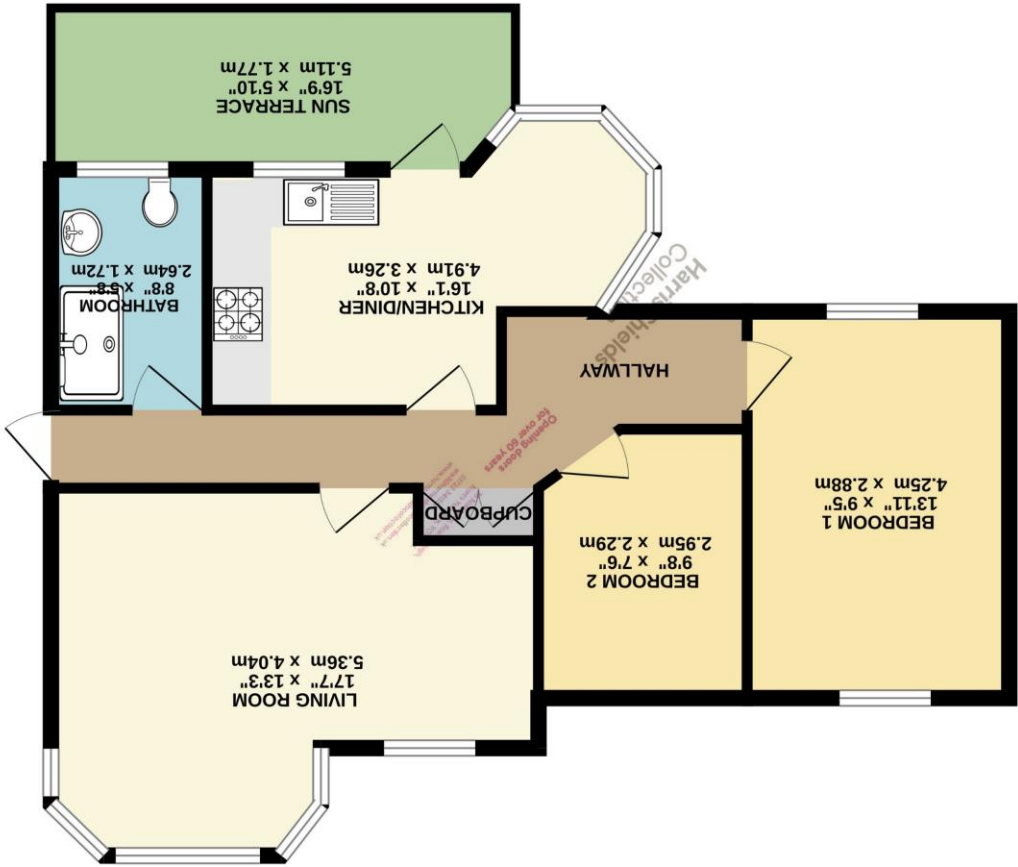
GROUND FLOOR 666 sq.ft. (61.9 sq.m.) approx.
